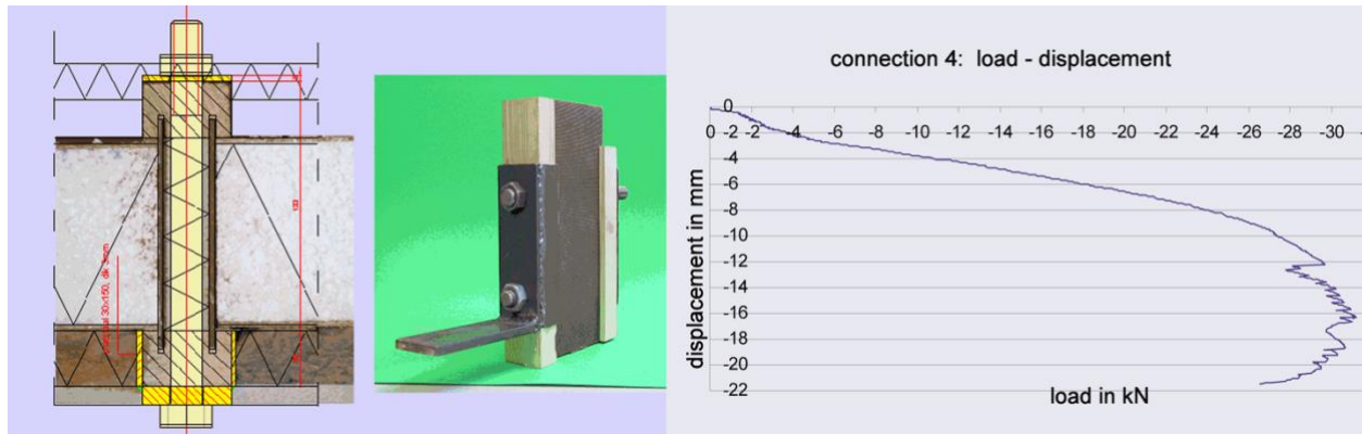
Figure 4: Concept of connection to transfer heavy loads in the small studs of the wall panel.
