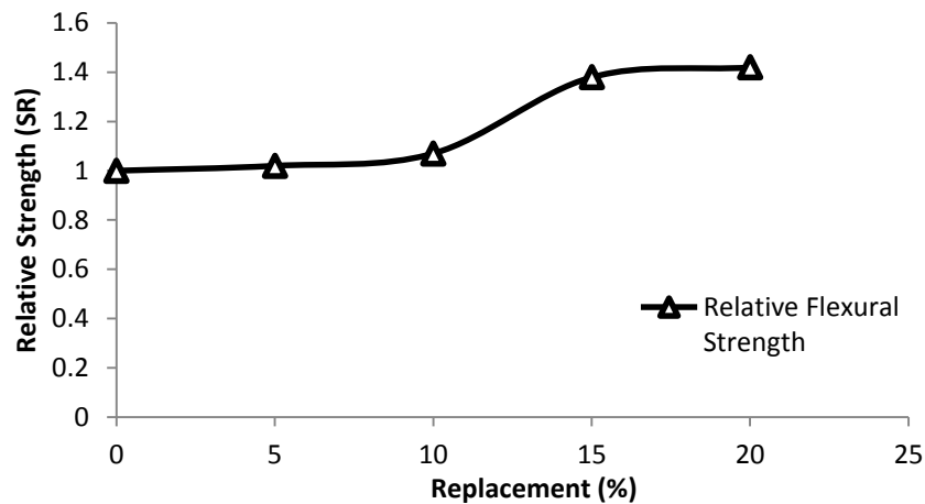
Figure 10: Relative Comparison of Flexural Strength
