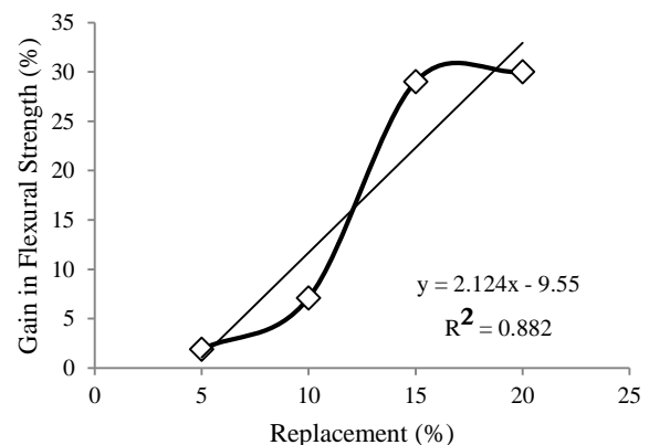
Figure 7: Gain in Flexural Strength Vs Replacement
