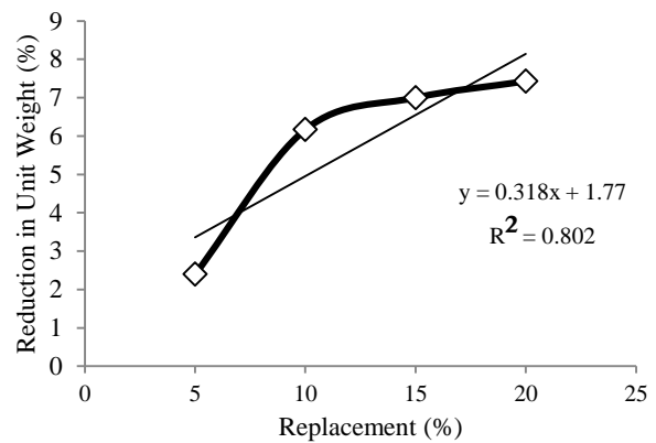
Figure 5: Reduction in unit weight Vs Replacement
