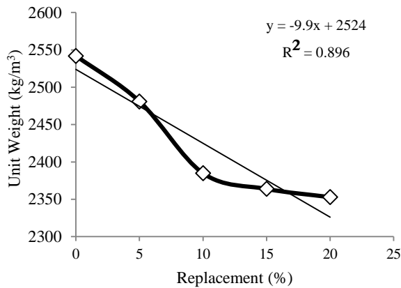
Figure 4: Unit Weight Vs Replacement
