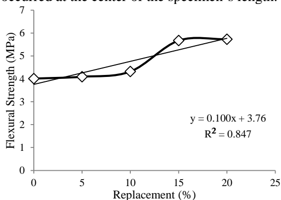
Figure 6: Flexural Strength Vs Replacement
