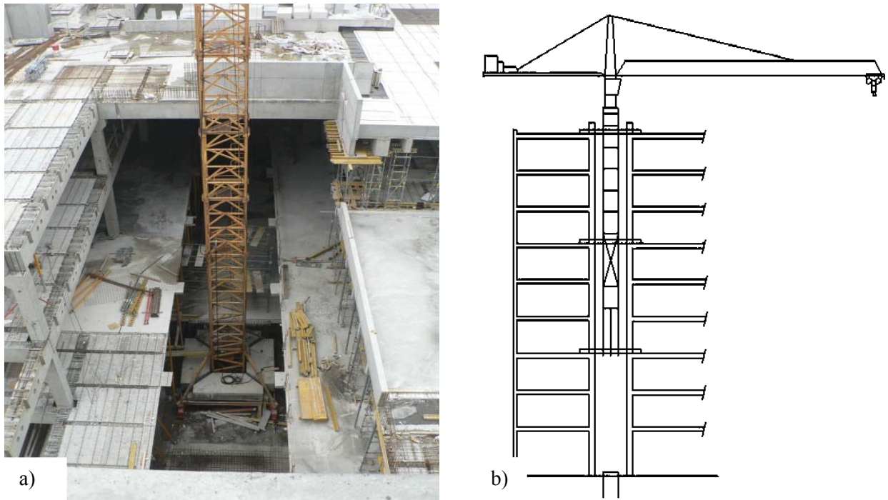
Figure 3: a) Crane Positioning onto Terrain within Structure Floor Plan – Aupark Bratislava b) Scansorial Crane Scheme
