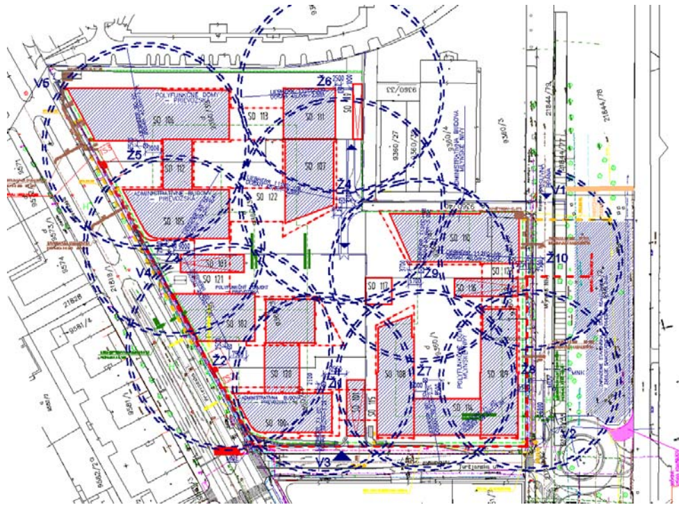
Figure 1: Tower Cranes Plan – Multifunctional Complex Apollo 2 Bratislava
