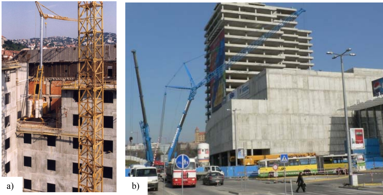
Figure 4: a) Crane on Ceiling Structure of the 6 th Floor – Carlton Bratislava b) Removal of Crane Tower from Structure – Aupark Bratislava
