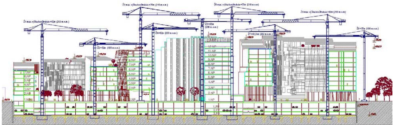
Figure 6: Vertical Arrangement of Tower Cranes – RIVER PARK Bratislava
